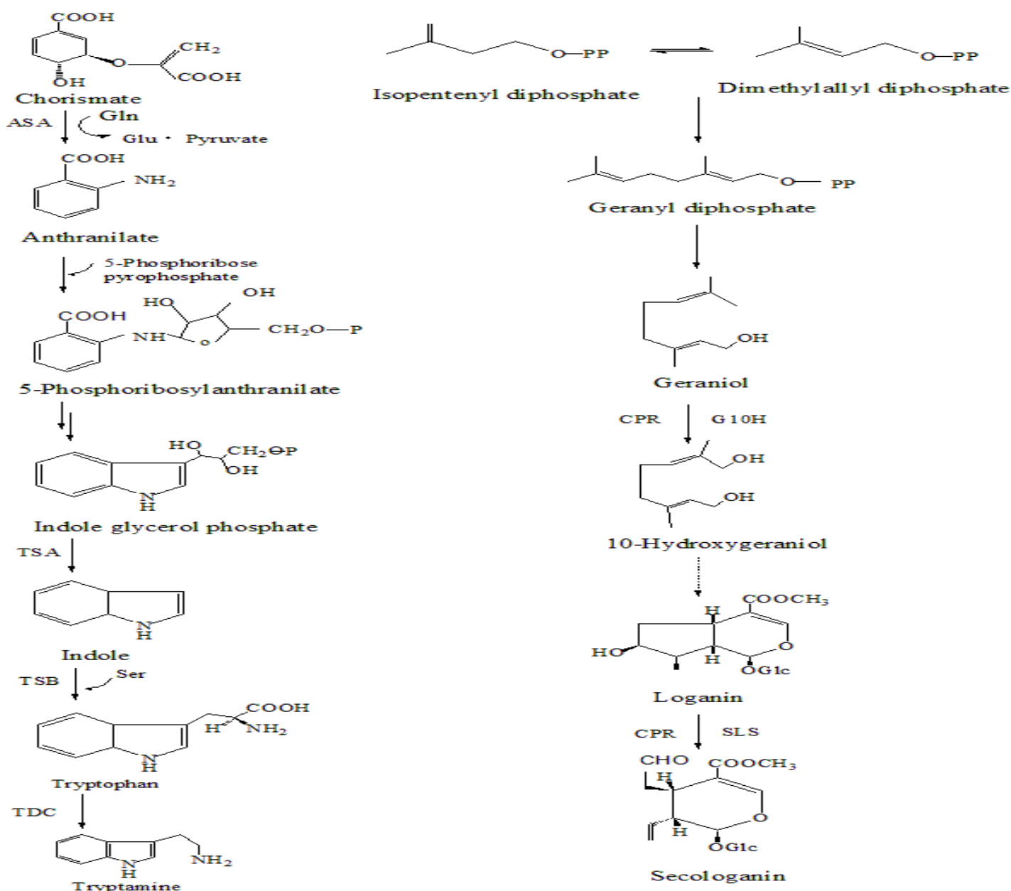
Fig. 2: Biosynthetic pathway of Tryptamine and Secologanin
