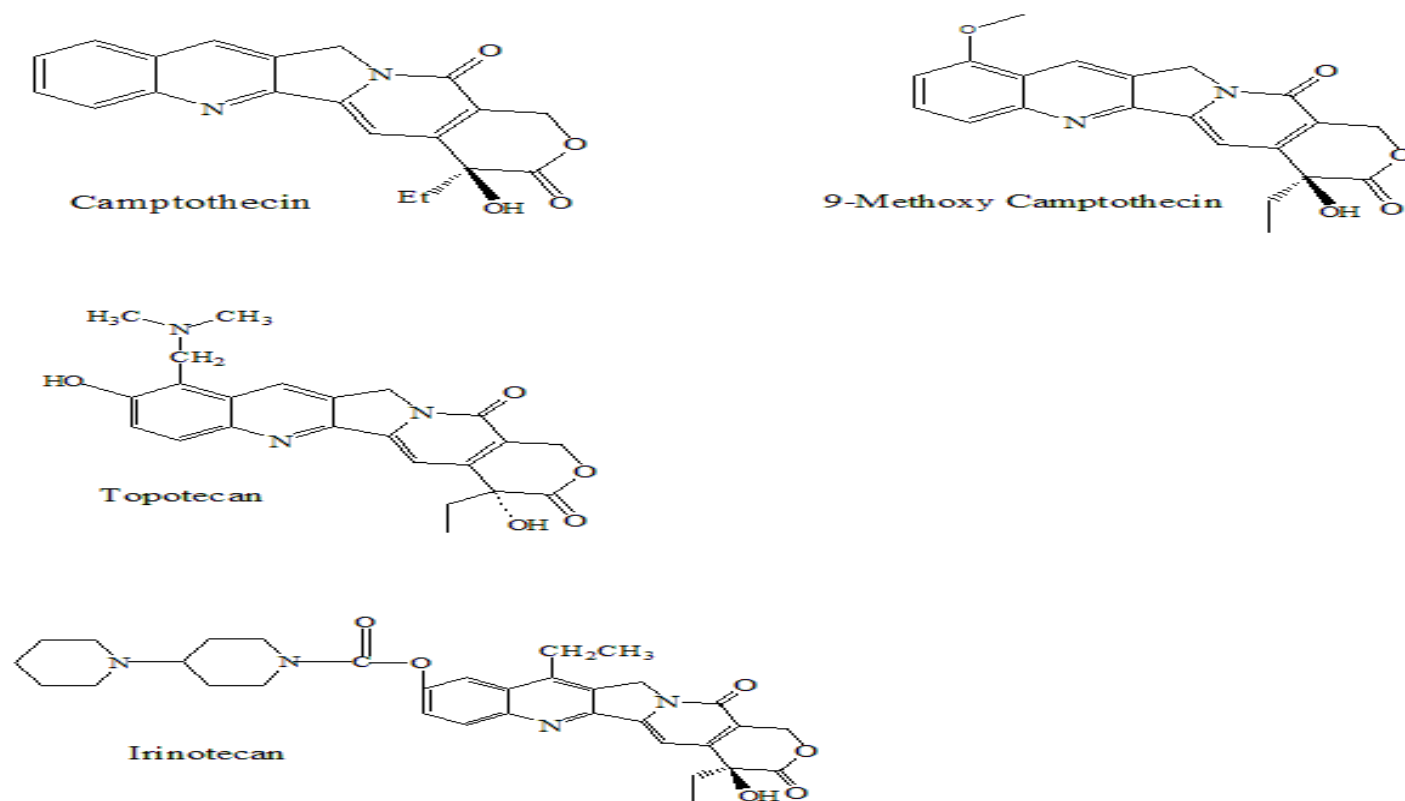
Fig. 1: Structure of CPT and its derivatives
